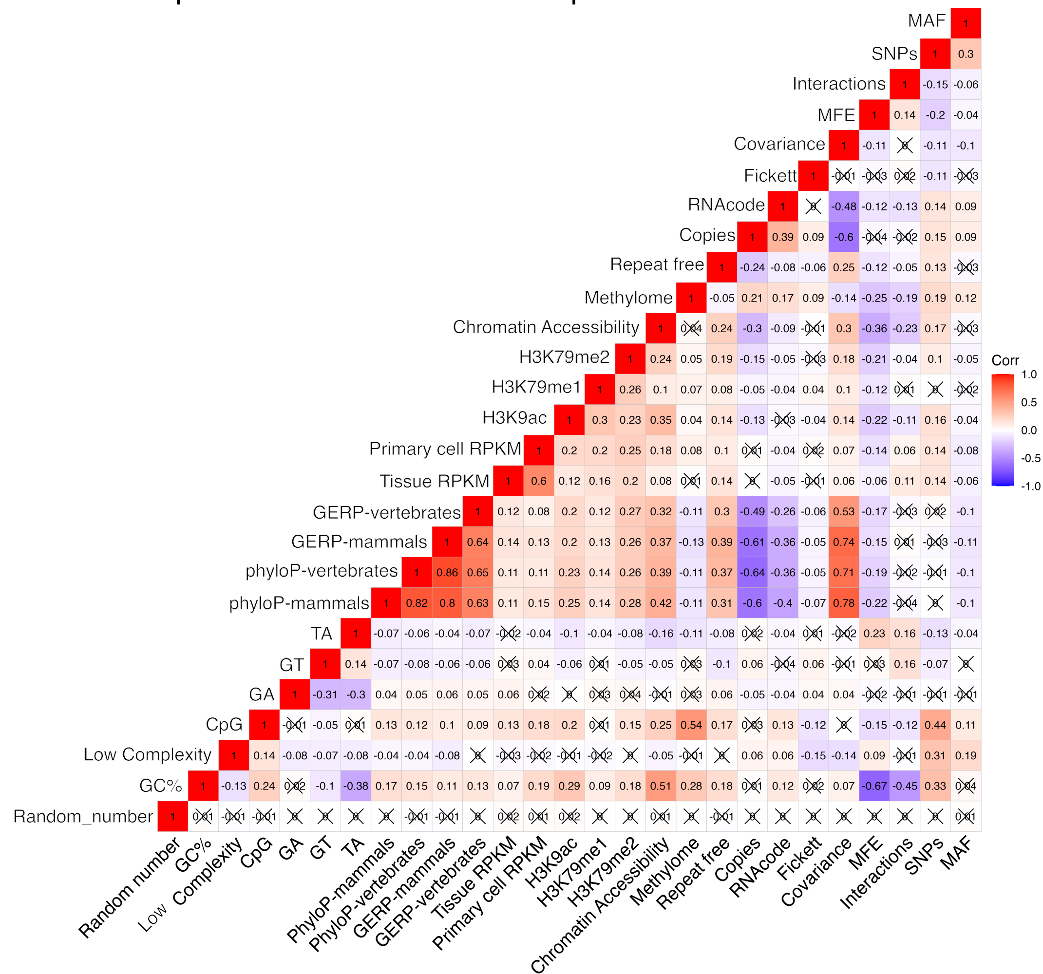
Supplementary Figure S2. sncRNA correlation matrix. Spearman correlation of functionality predictors for sncRNA sequences. Positively correlated features are displayed in red and negatively correlated features in blue. Spearman's Rho was used to determine the significance of each correlation, which were corrected for multiple testing using a Bonferroni correction. Non-significant correlations with a p-value > 0.05 have been marked with a cross.
